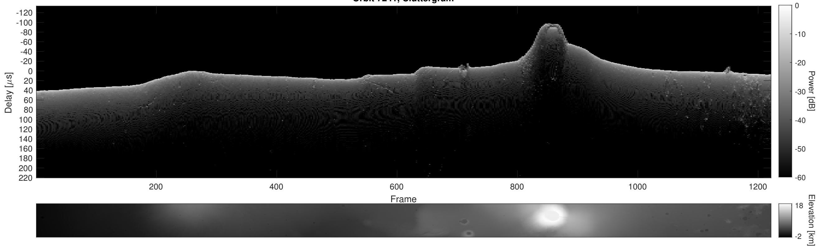
Orbit 7241, Cluttergram
