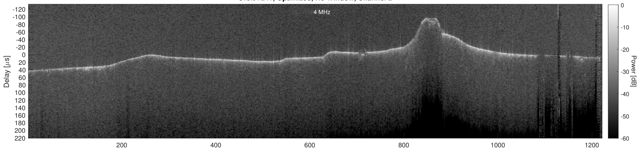
Orbit 7241, Cluttergram
