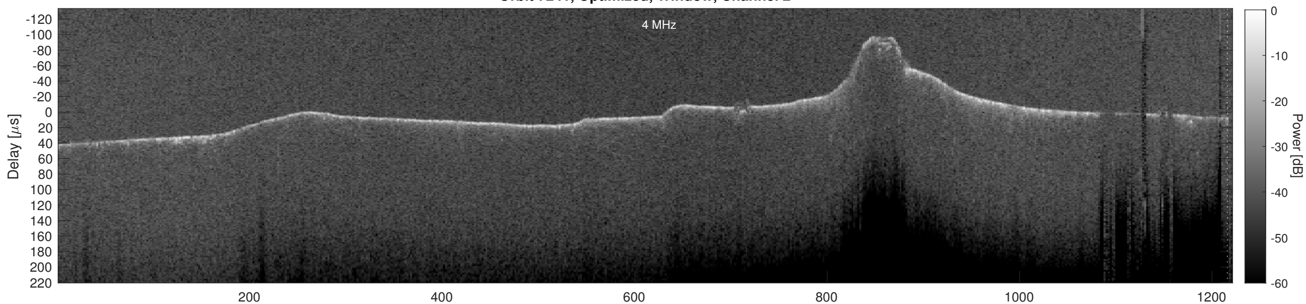
Orbit 7241, Cluttergram
