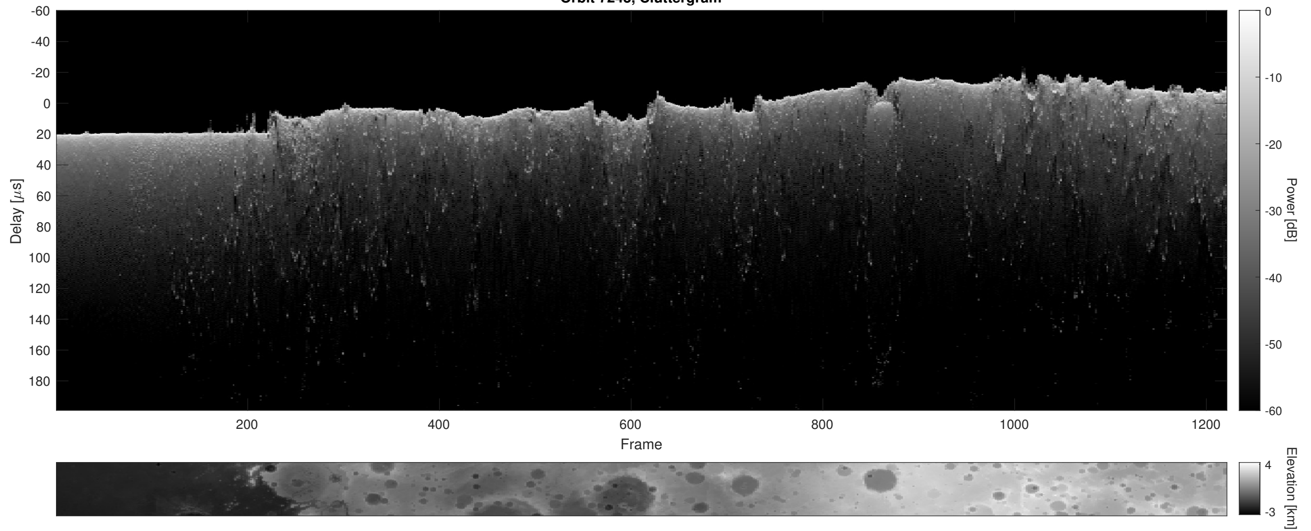
Orbit 7243, Cluttergram
