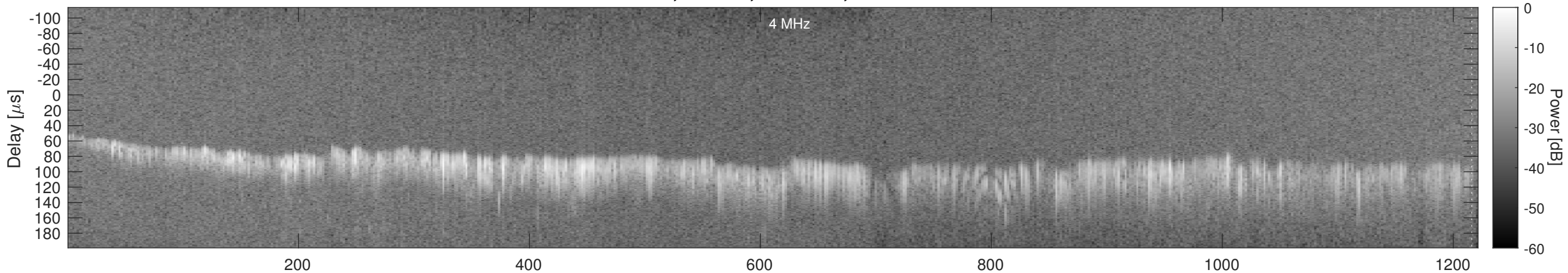
Orbit 7243, Window, Channel 2, Chapman
