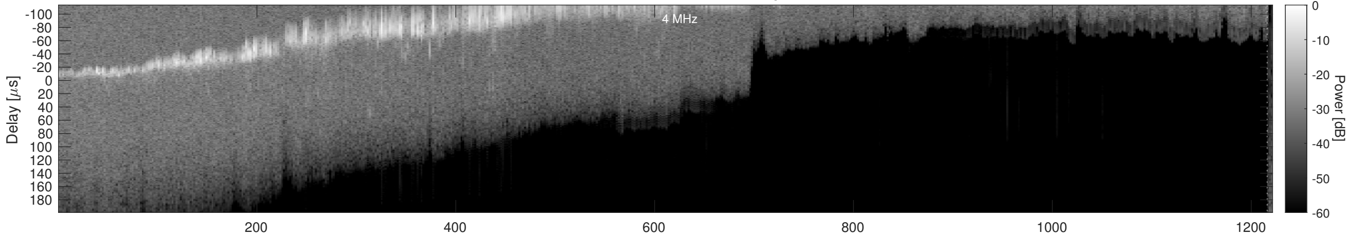
Orbit 7243, Window, Channel 2, Optimized
