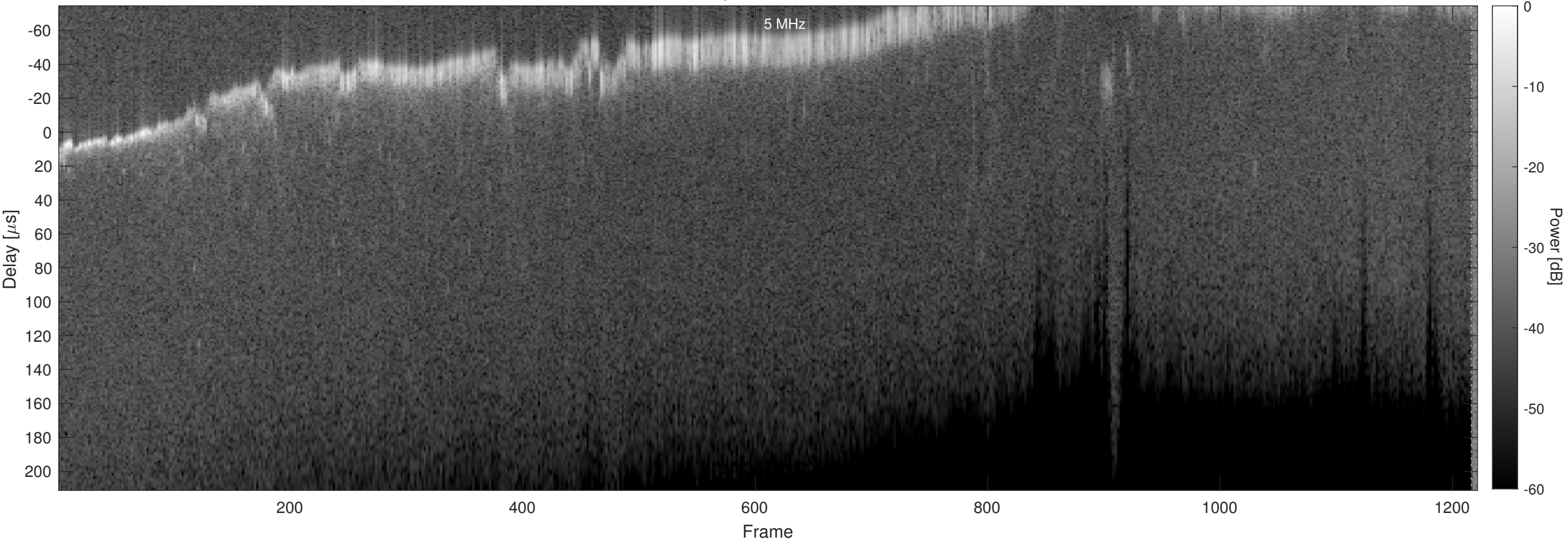
Orbit 7244, Chapman, Window, Channel 2
