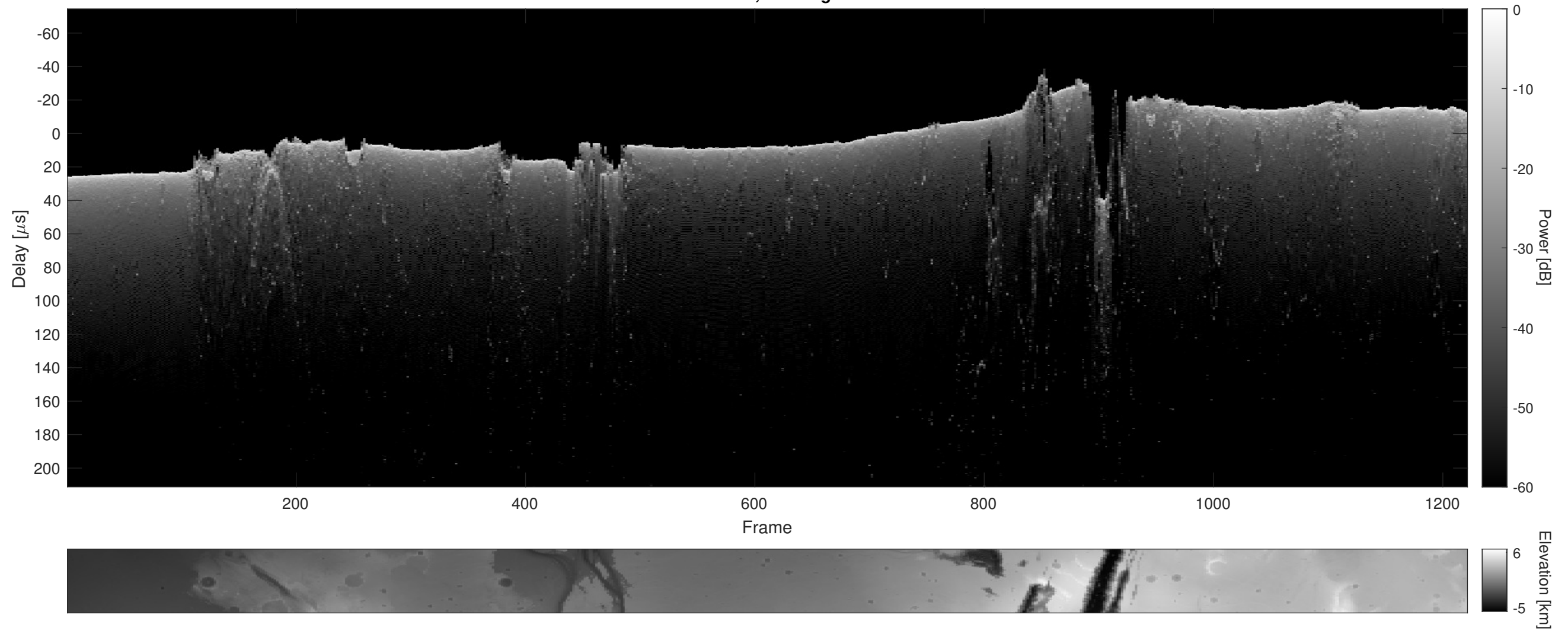
Orbit 7244, Cluttergram
