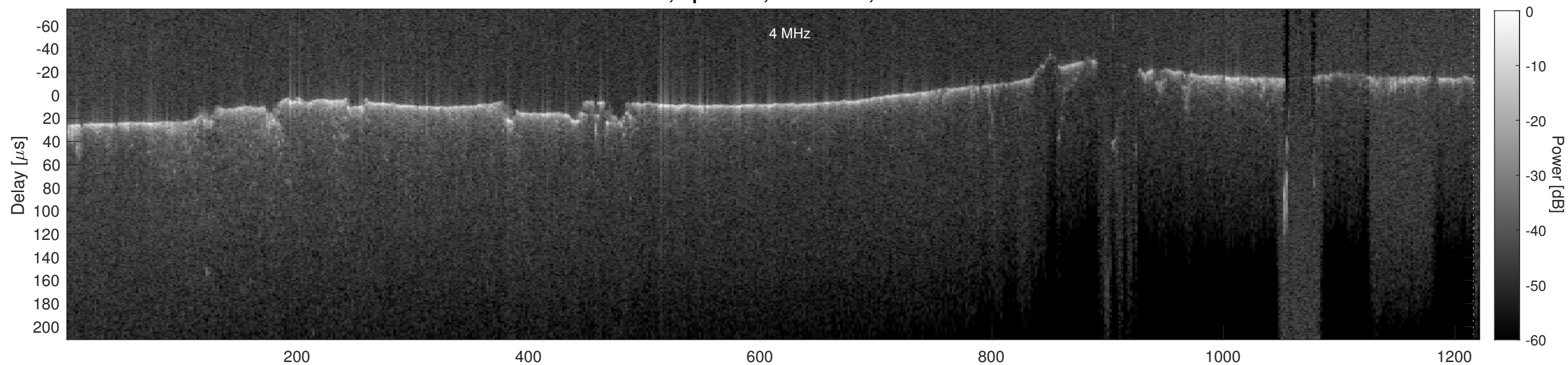
Orbit 7244, Cluttergram
