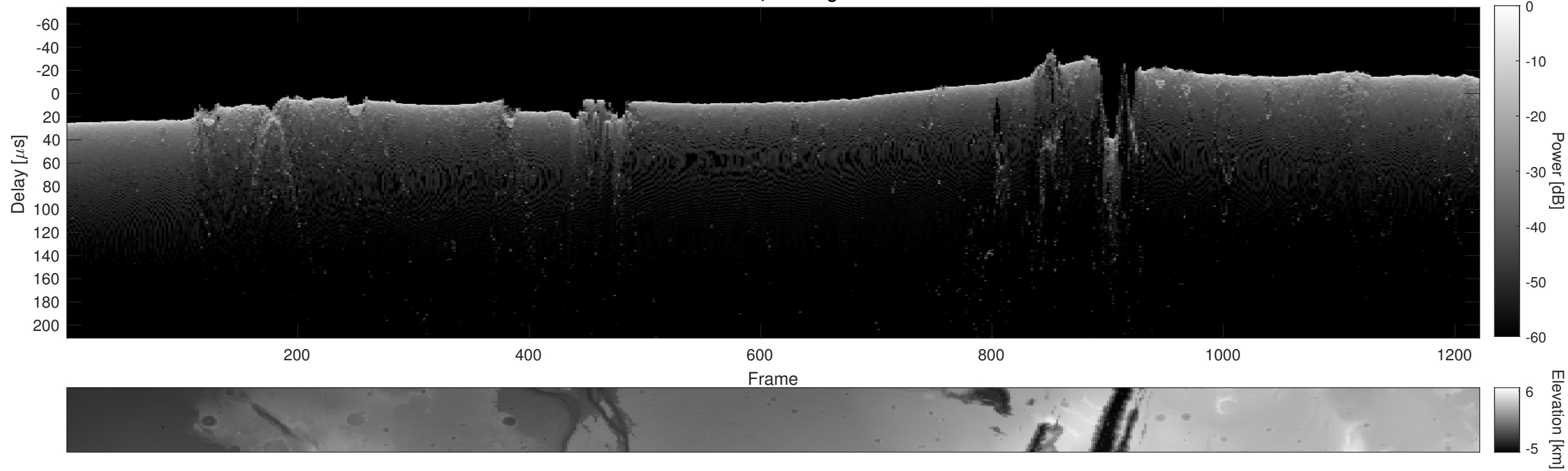
Orbit 7244, Cluttergram
