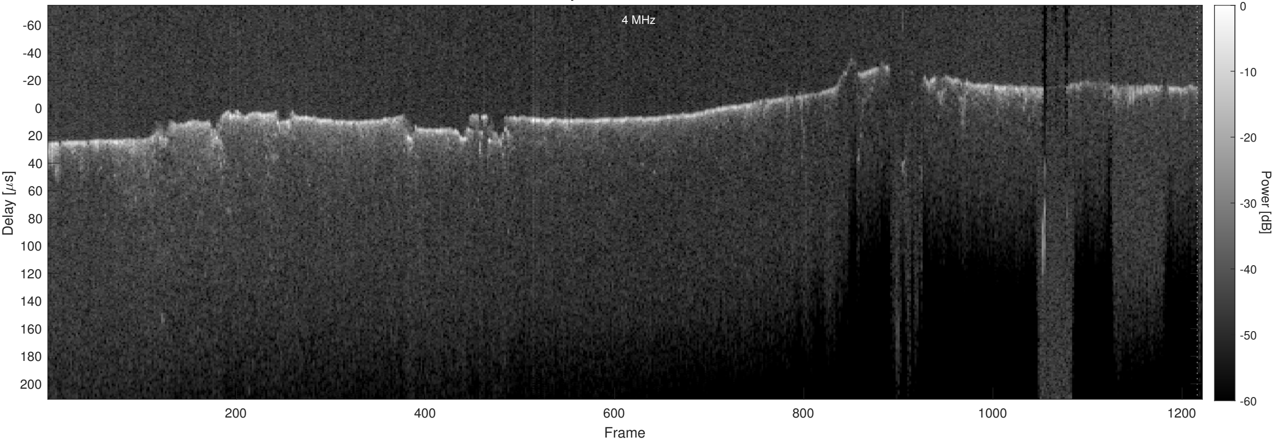
Orbit 7244, Optimized, Window, Channel 2
