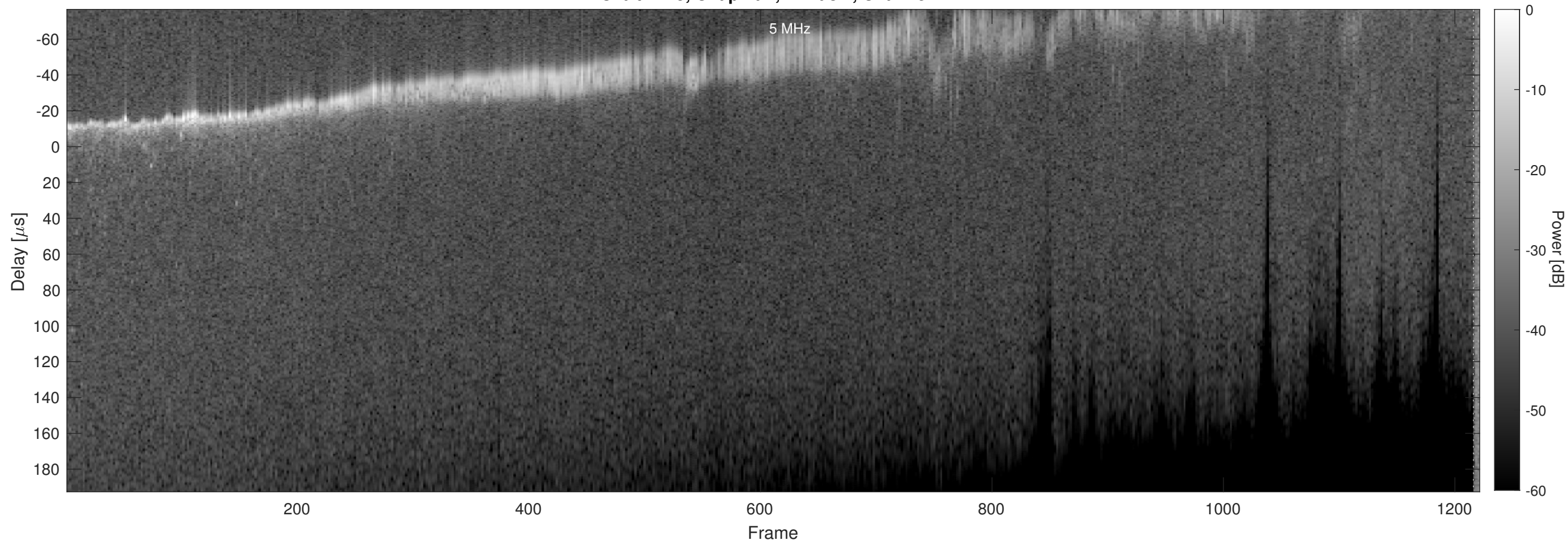
Orbit 7245, Chapman, Window, Channel 2
