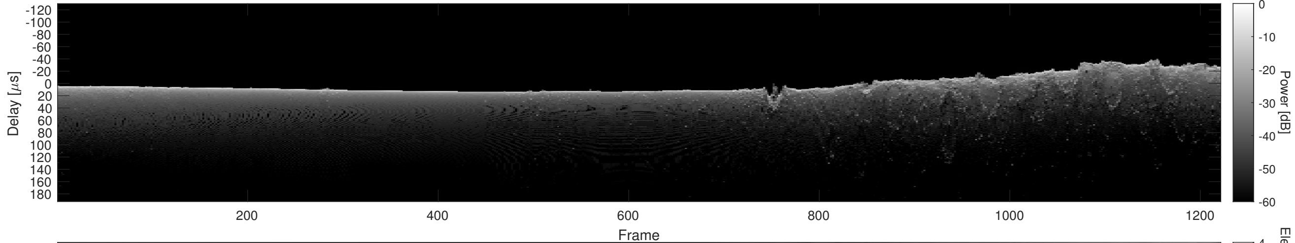
Orbit 7245, Cluttergram
