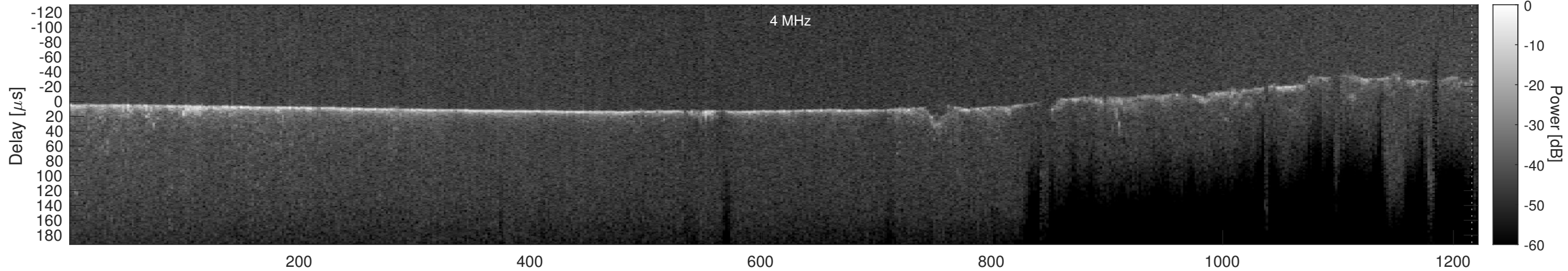
Orbit 7245, Cluttergram
