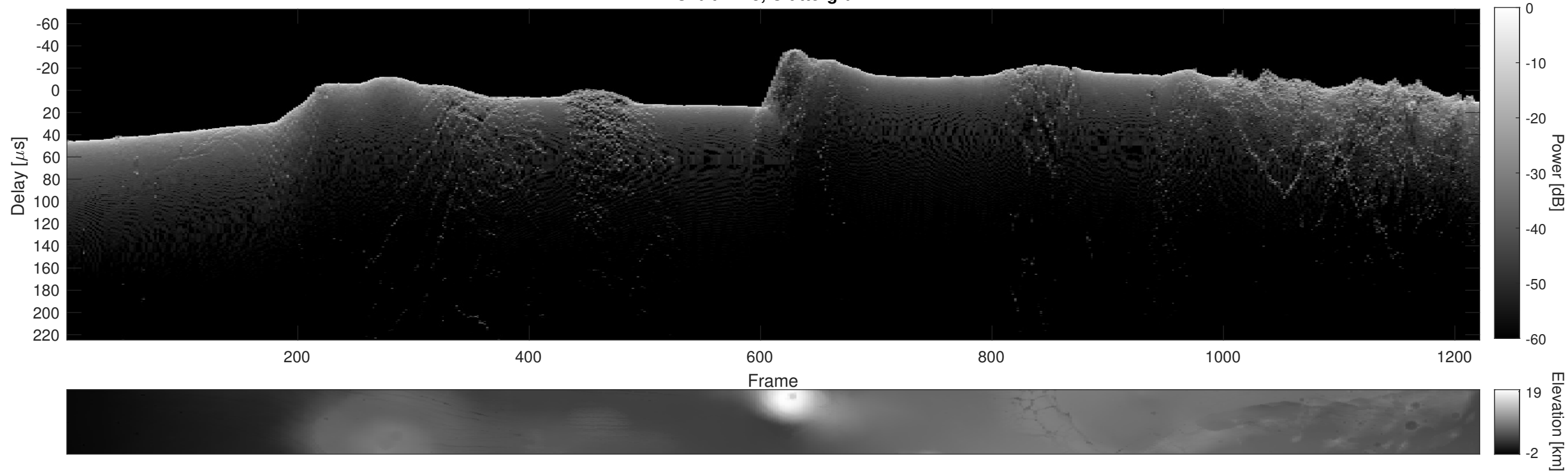
Orbit 7248, Cluttergram
