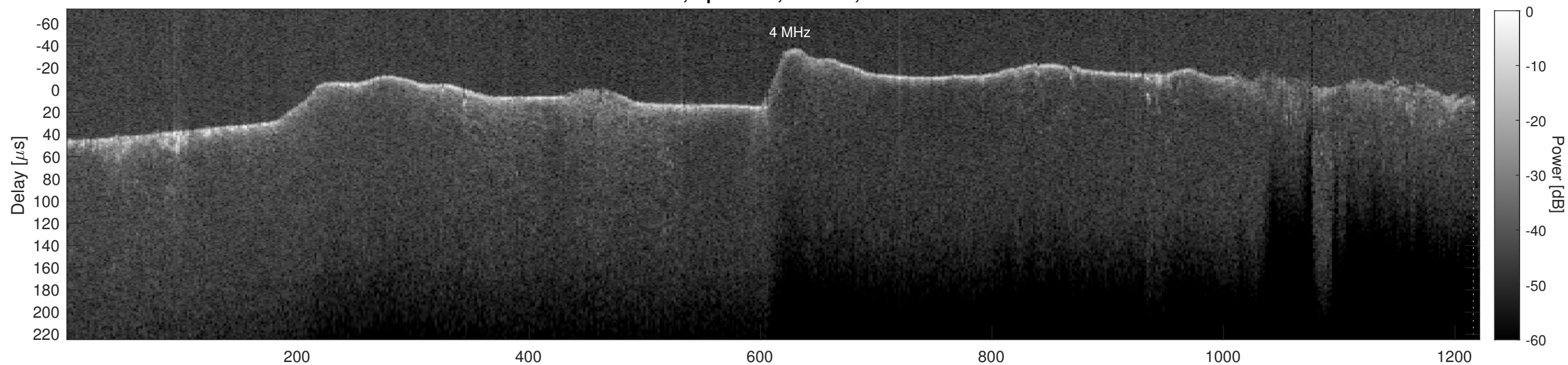
Orbit 7248, Cluttergram
