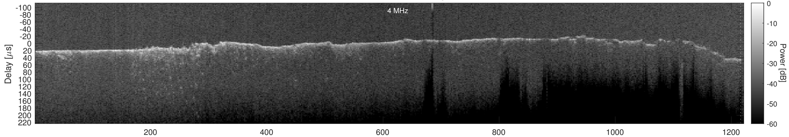
Orbit 7250, Cluttergram
