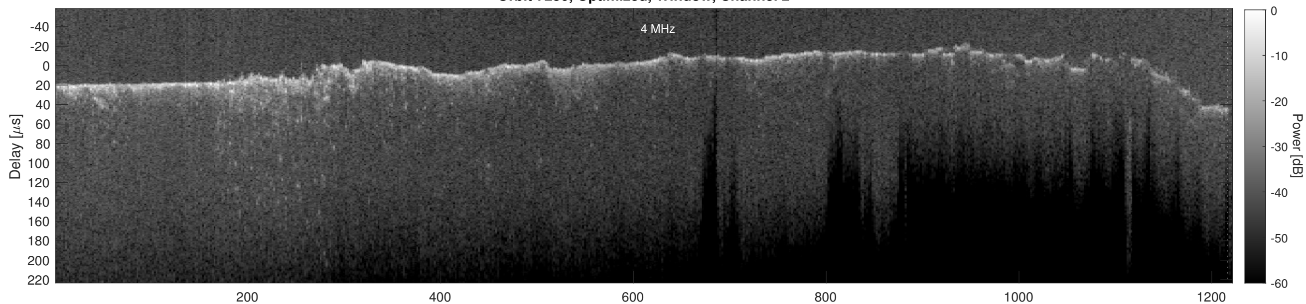
Orbit 7250, Cluttergram
