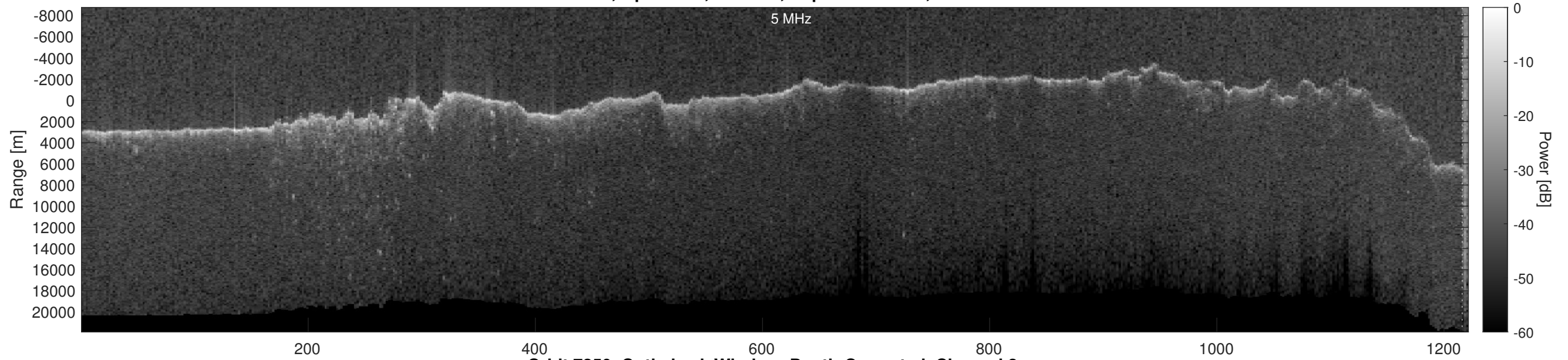
Orbit 7250, Optimized, Window, Depth-Corrected, Channel 2
