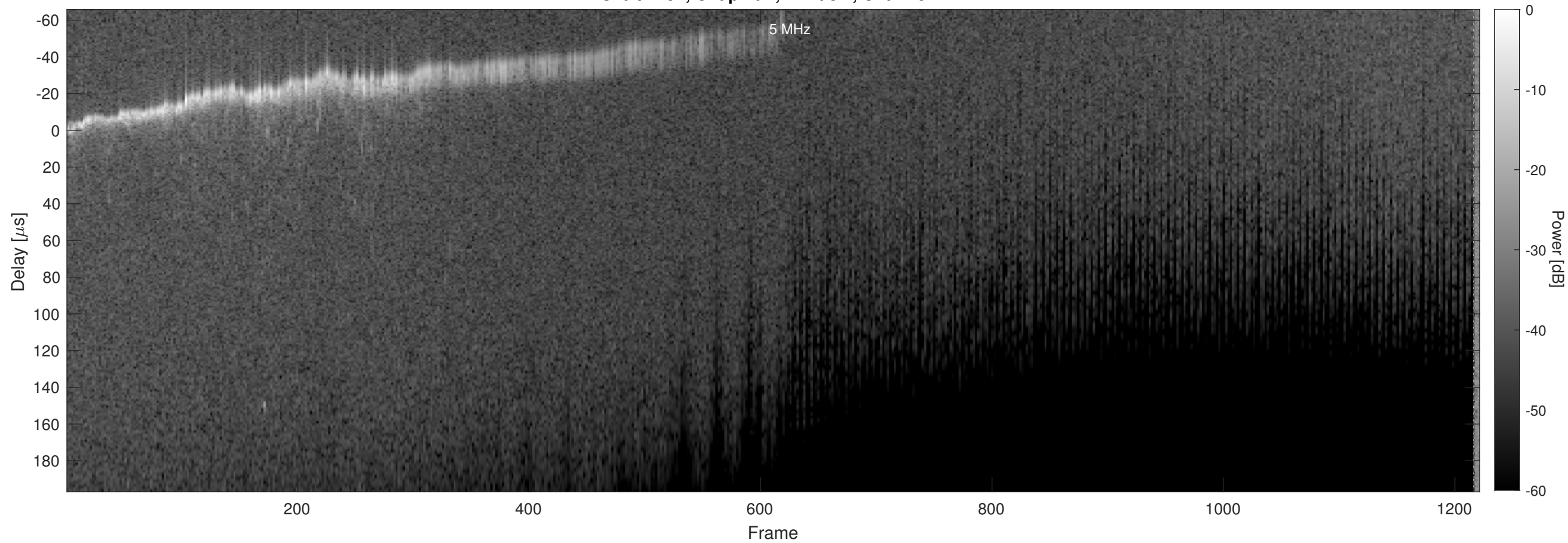
Orbit 7251, Chapman, Window, Channel 2
