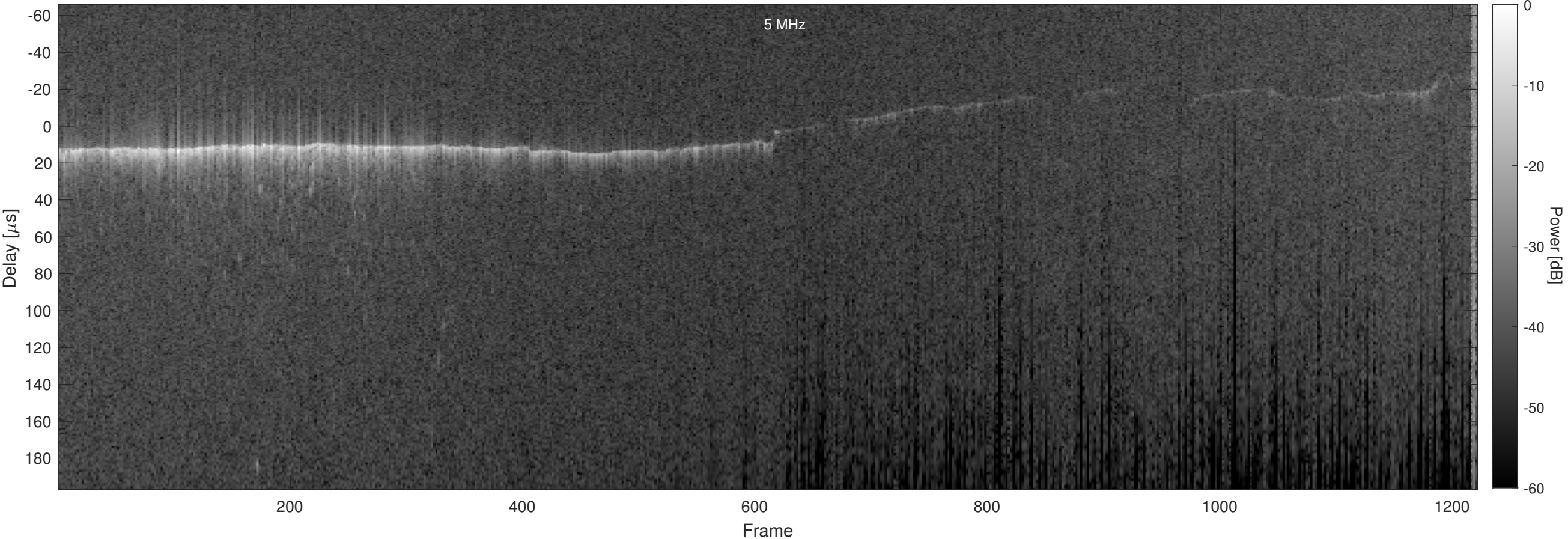
Orbit 7251, Optimized, No Window, Channel 2
