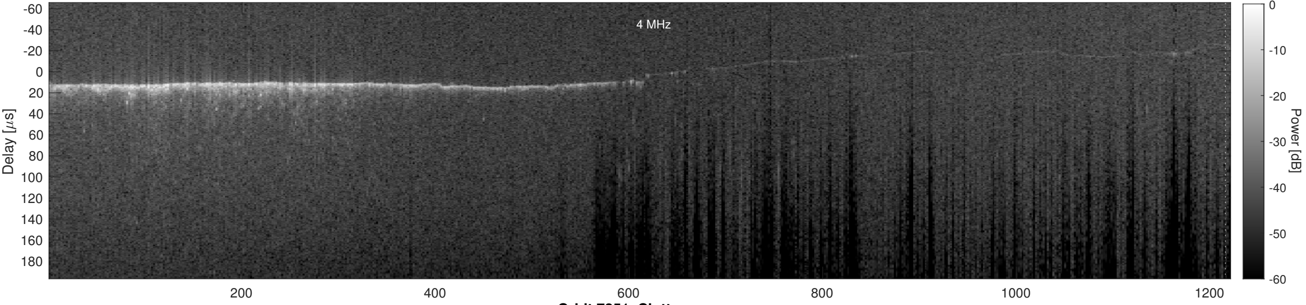
Orbit 7251, Cluttergram
