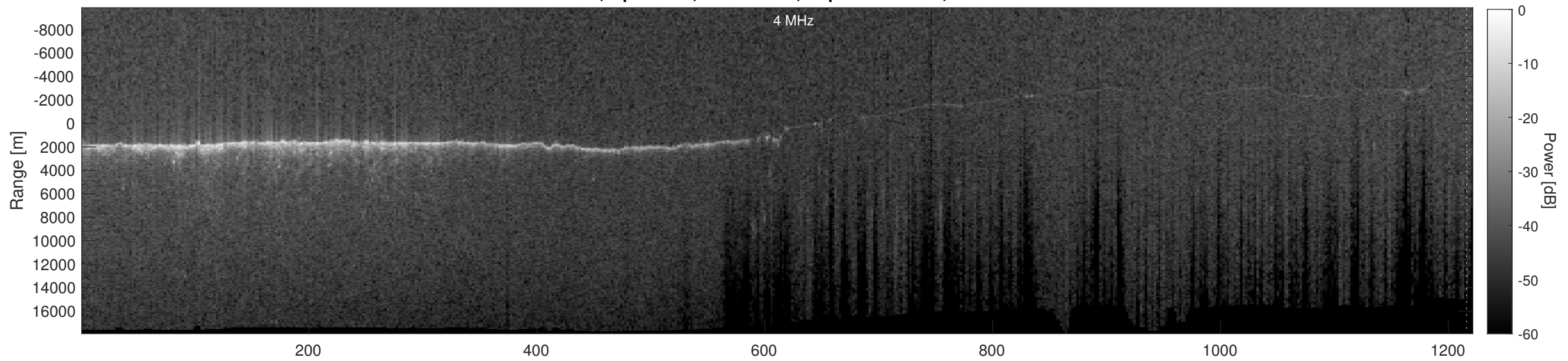
Orbit 7251, Depth-Corrected Cluttergram
