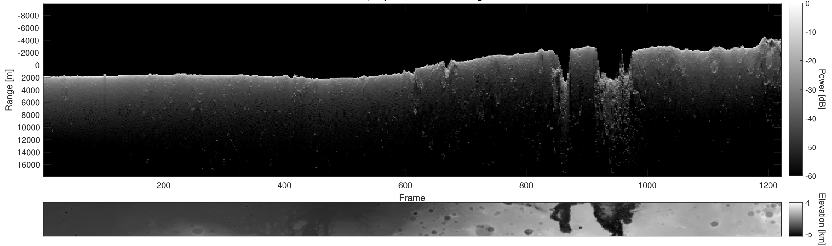
Orbit 7251, Depth-Corrected Cluttergram
