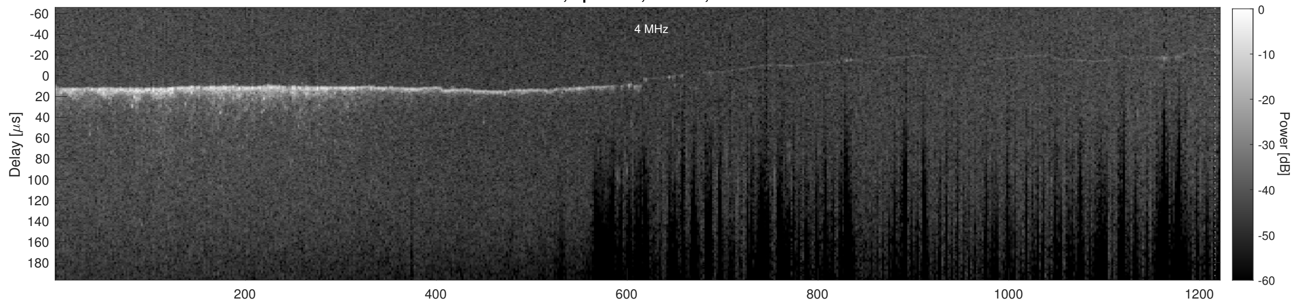
Orbit 7251, Cluttergram
