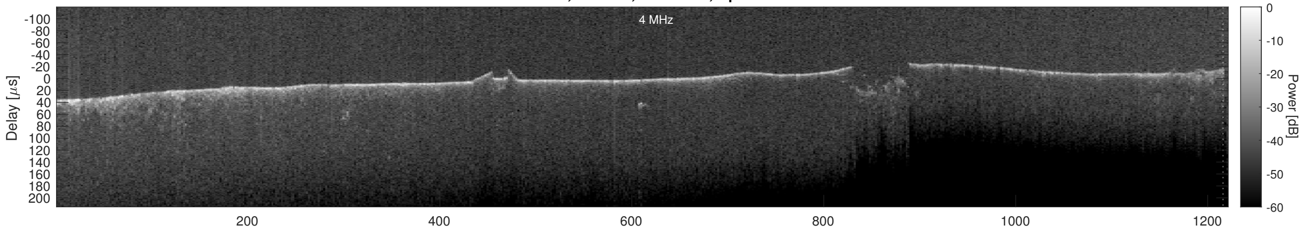
Orbit 7255, Cluttergram
