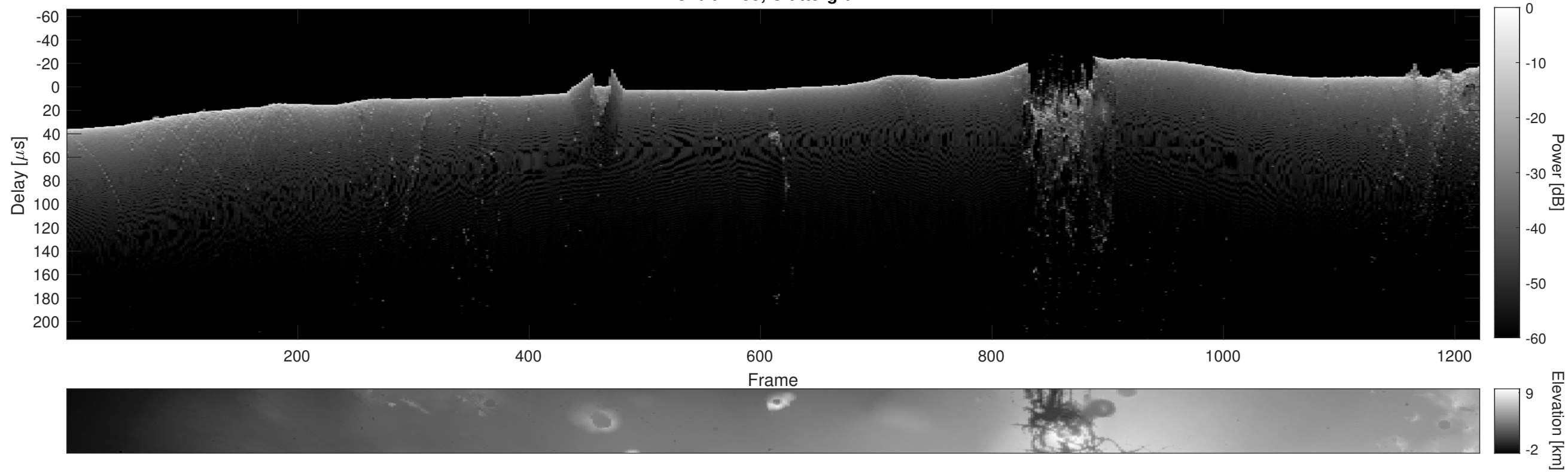
Orbit 7255, Cluttergram
