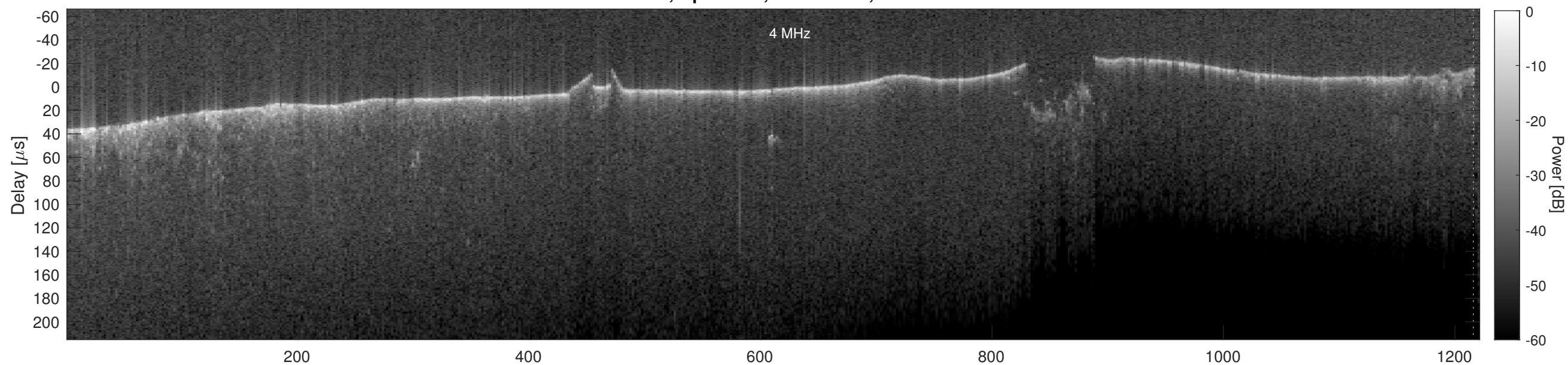
Orbit 7255, Cluttergram
