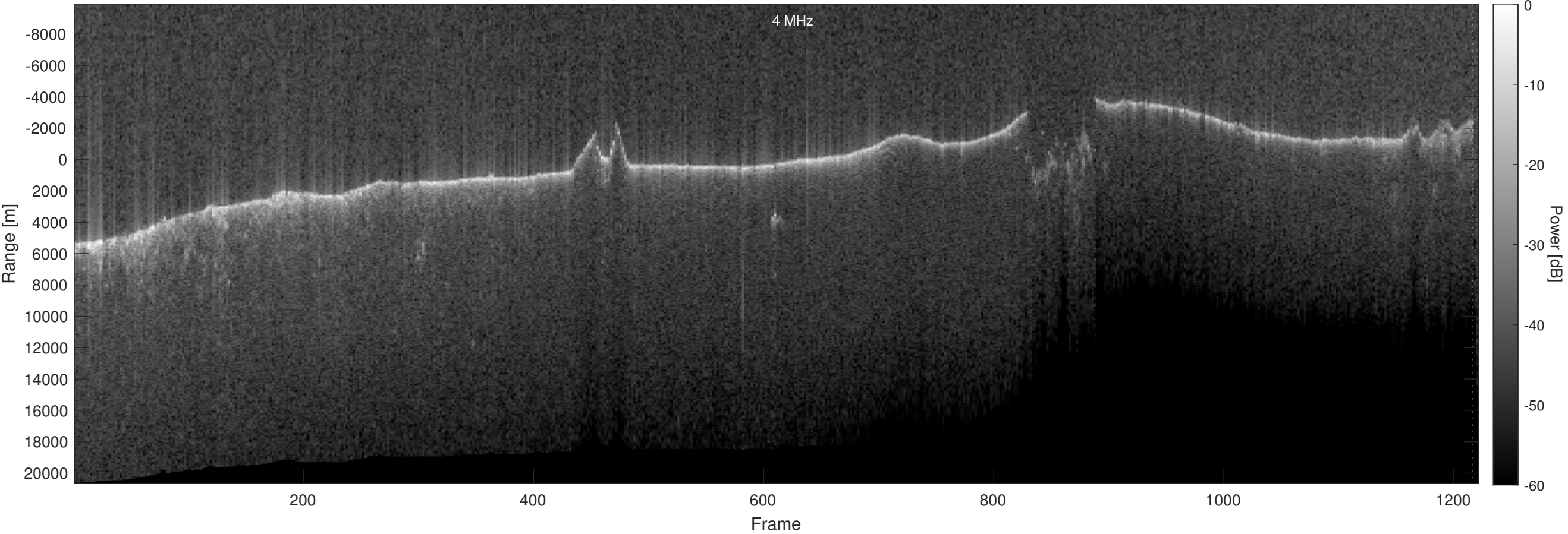
Orbit 7255, Optimized, No Window, Depth-Corrected, Channel 2
