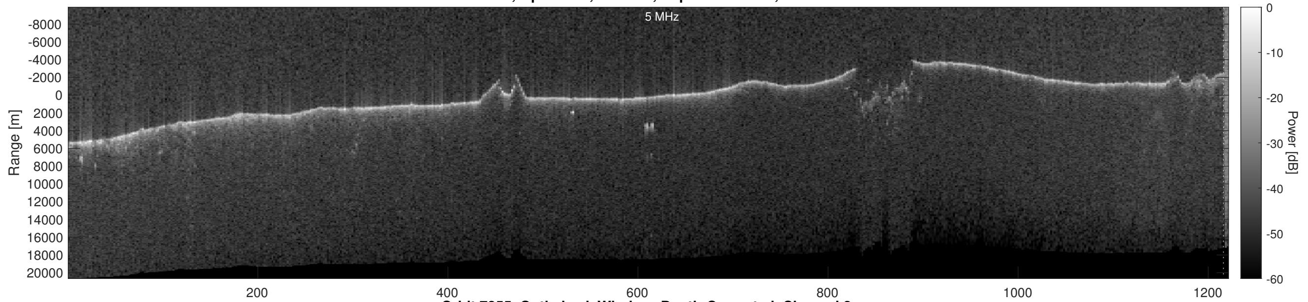
Orbit 7255, Optimized, Window, Depth-Corrected, Channel 2
