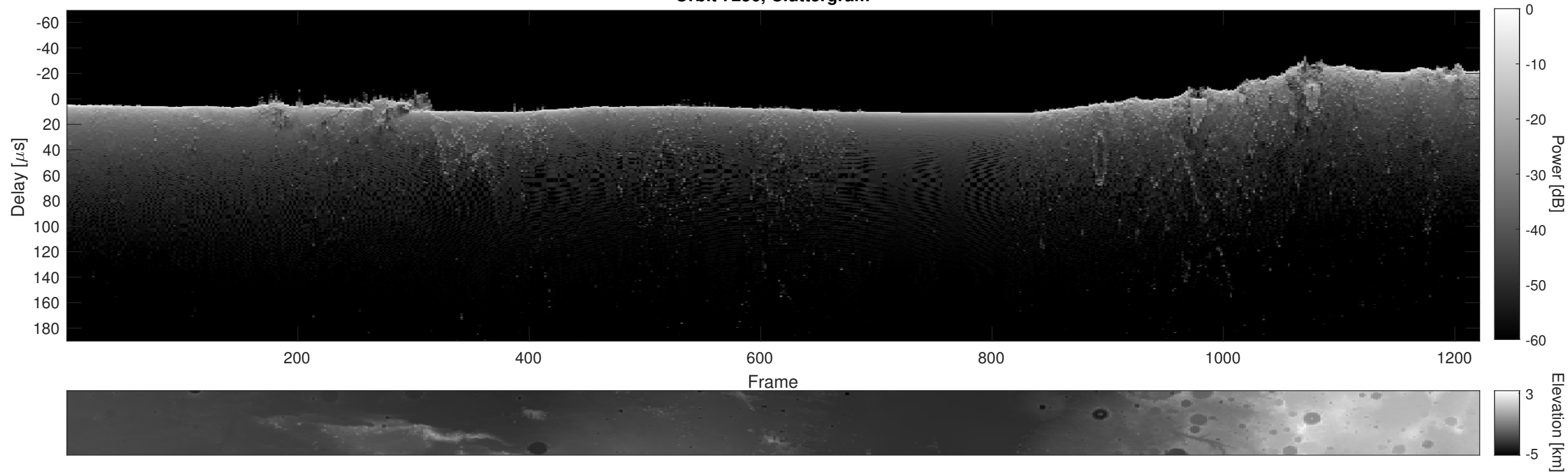
Orbit 7256, Cluttergram
