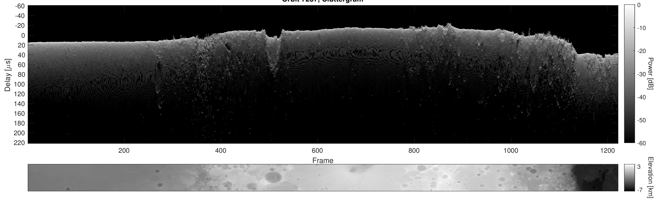
Orbit 7257, Cluttergram
