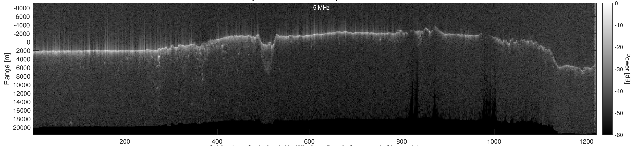
Orbit 7257, Optimized, No Window, Depth-Corrected, Channel 2
