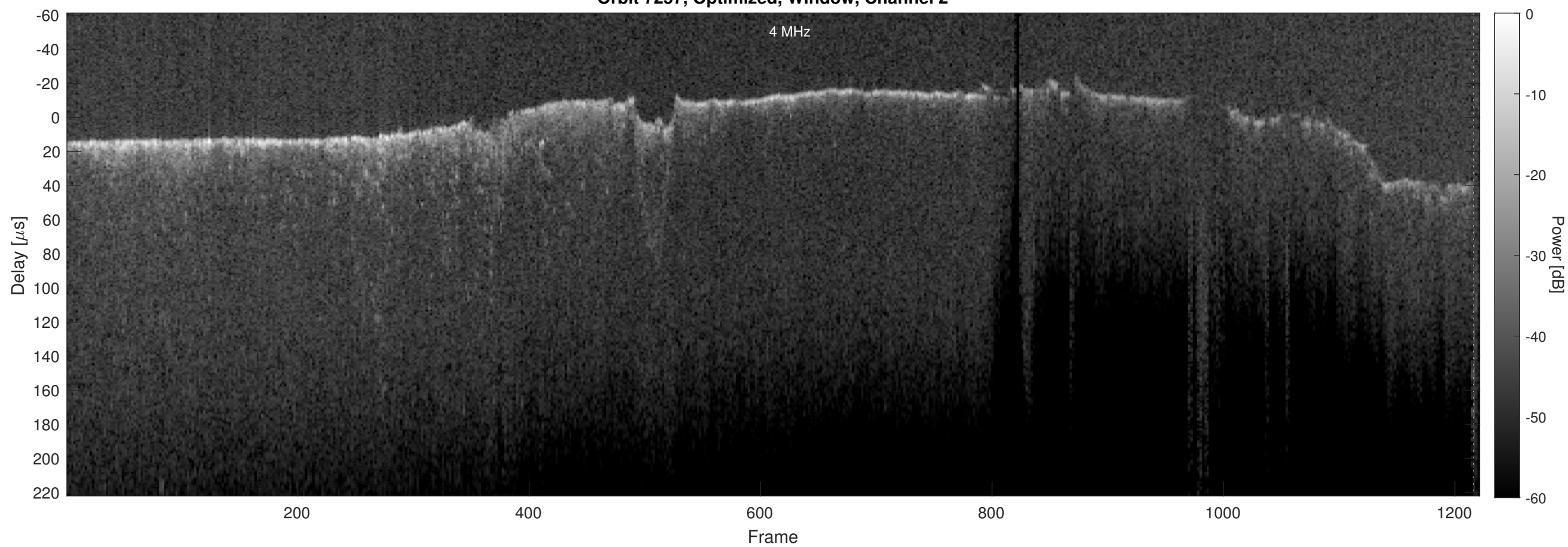
Orbit 7257, Optimized, Window, Channel 2
