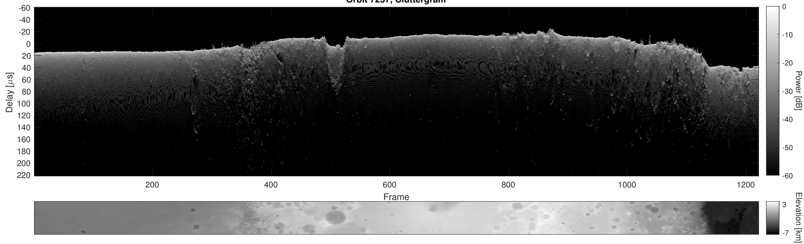
Orbit 7257, Cluttergram
