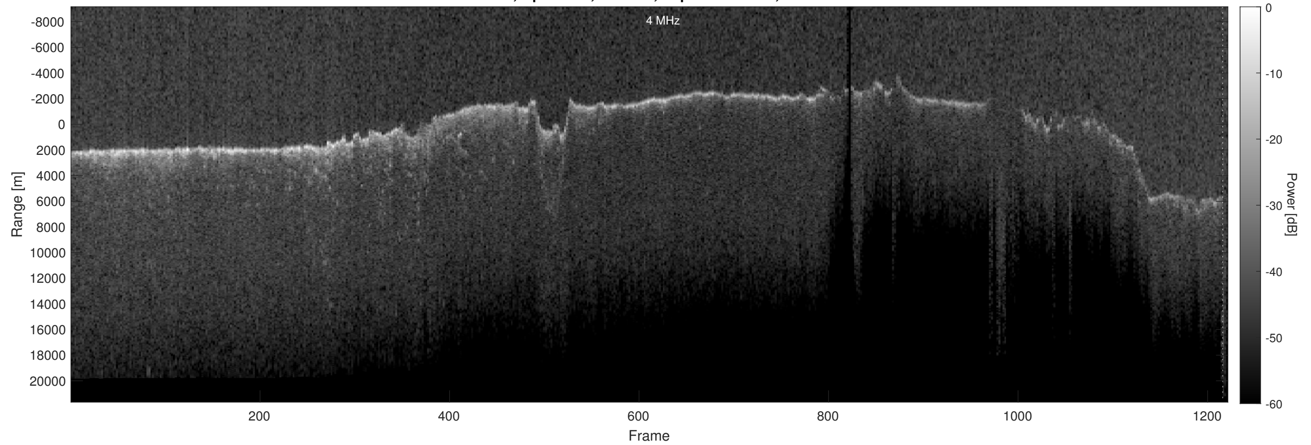
Orbit 7257, Optimized, Window, Depth-Corrected, Channel 2
