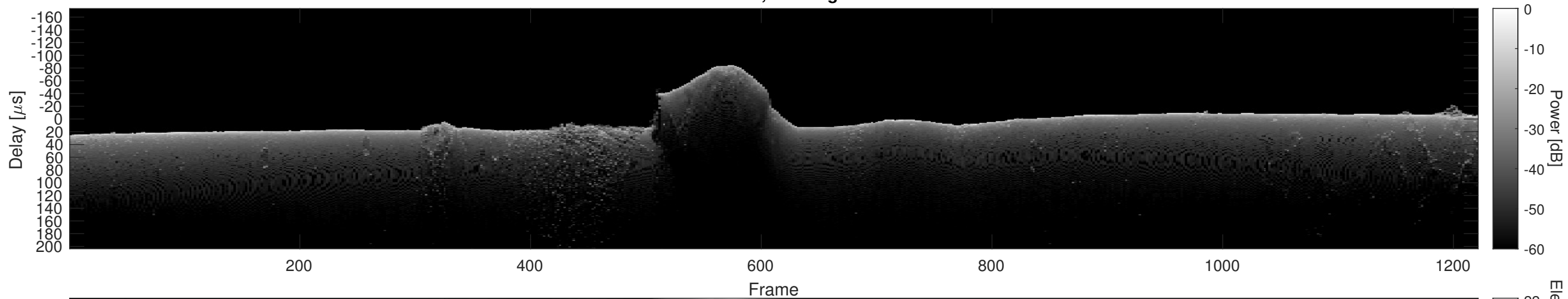
Orbit 7259, Cluttergram
