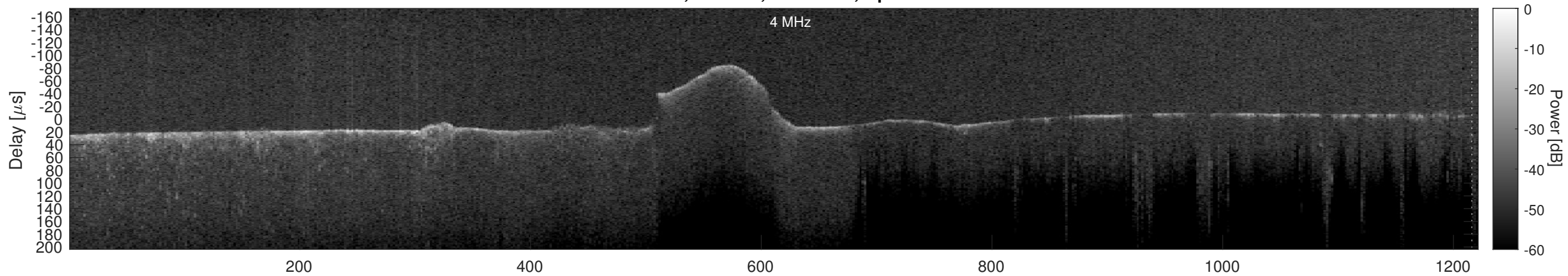
Orbit 7259, Cluttergram
