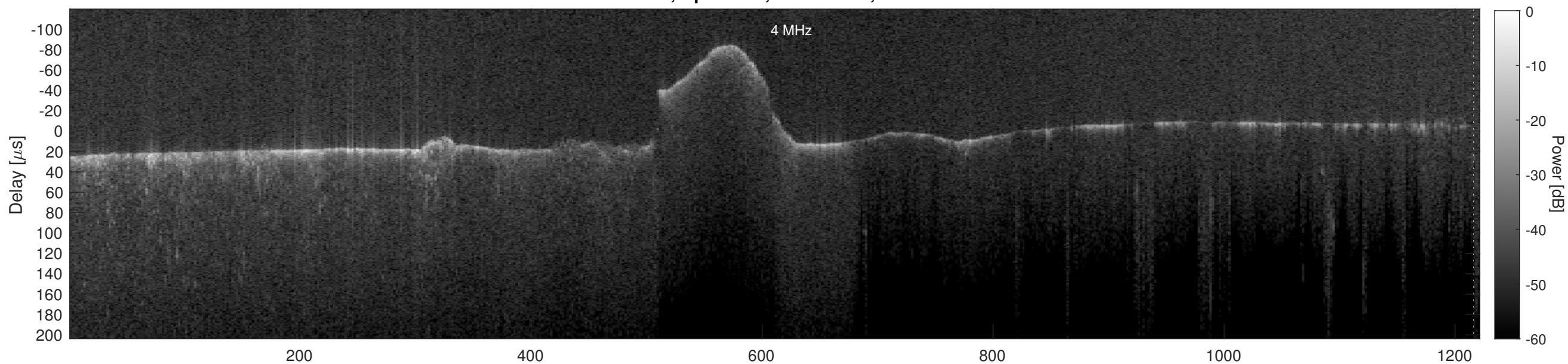
Orbit 7259, Cluttergram
