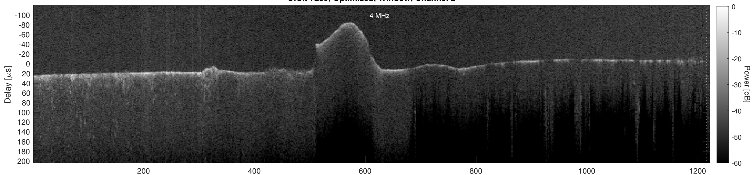
Orbit 7259, Cluttergram
