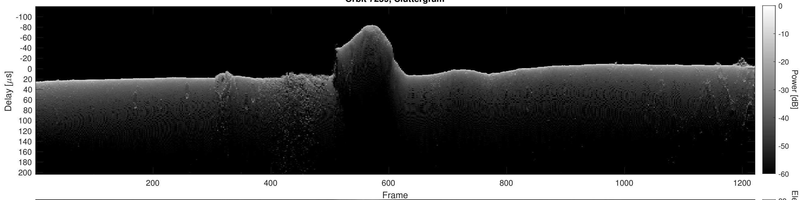
Orbit 7259, Cluttergram
