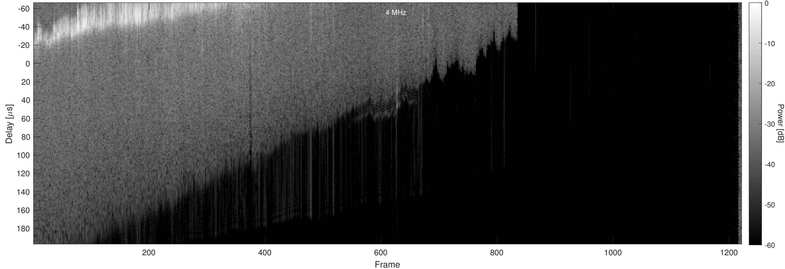
Orbit 7260, Chapman, No Window, Channel 2
