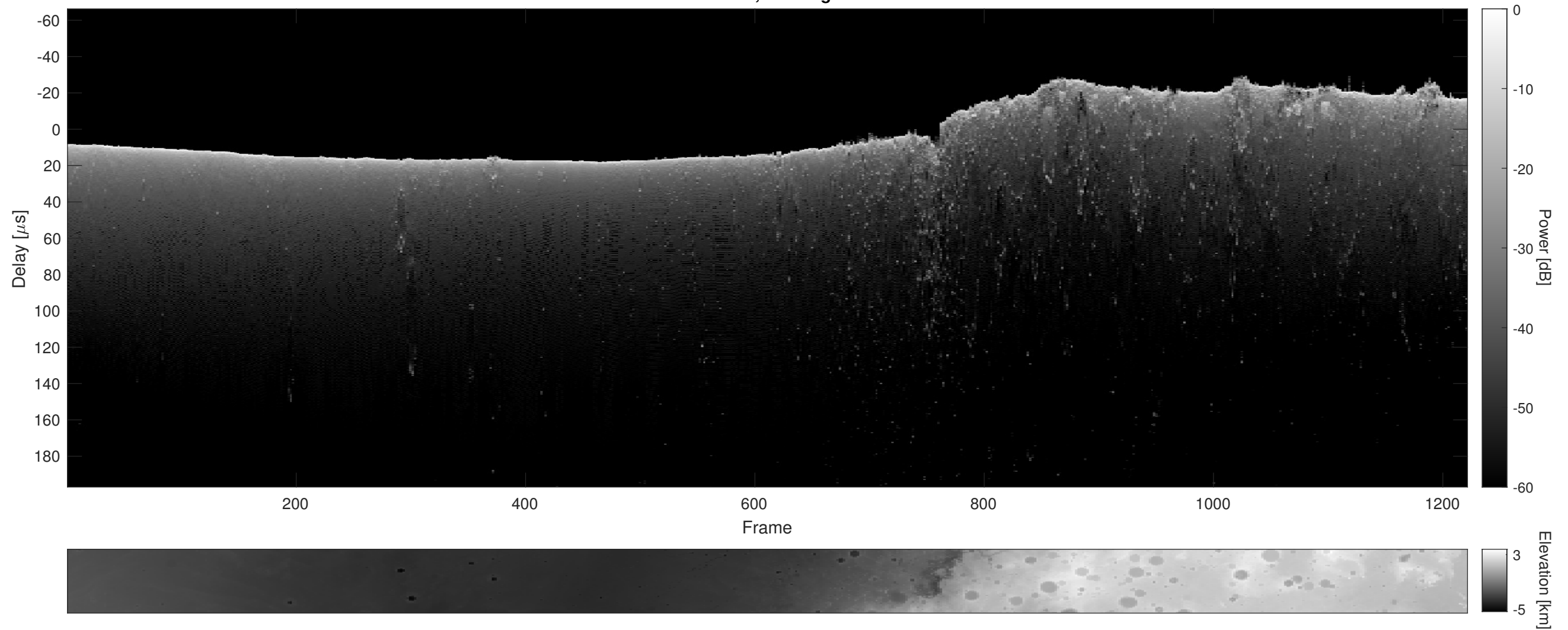
Orbit 7260, Cluttergram
