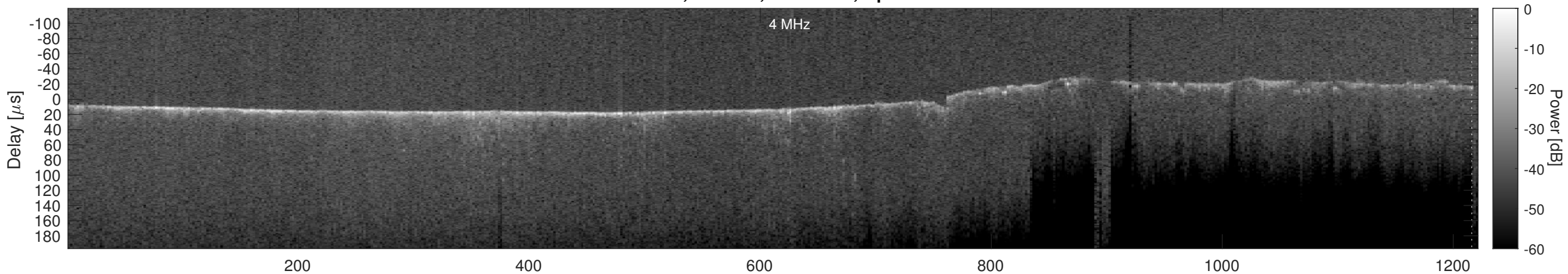
Orbit 7260, Cluttergram
