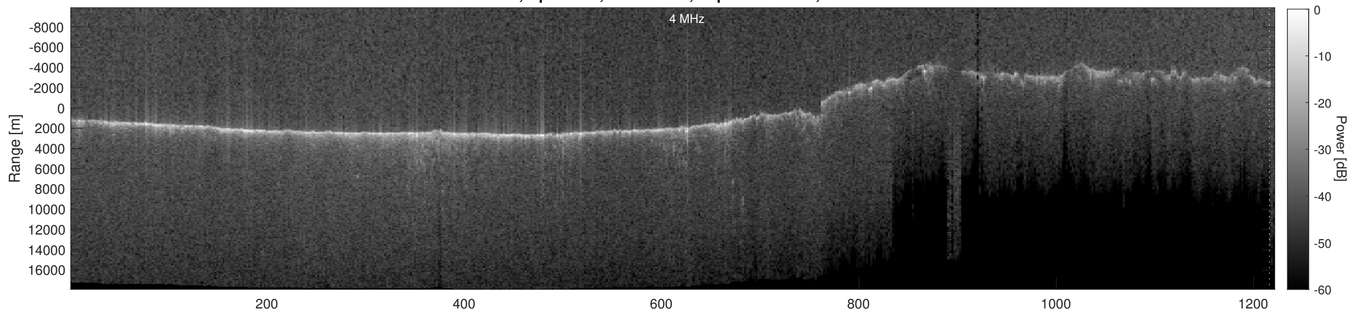
Orbit 7260, Depth-Corrected Cluttergram
