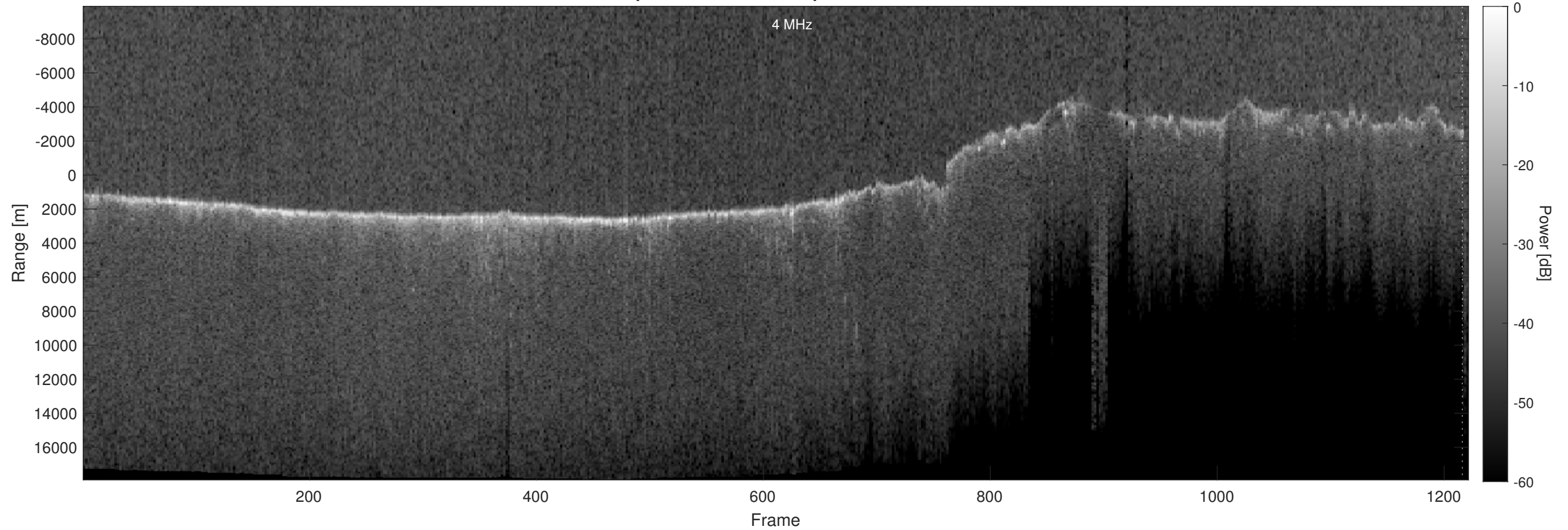
Orbit 7260, Optimized, Window, Depth-Corrected, Channel 2
