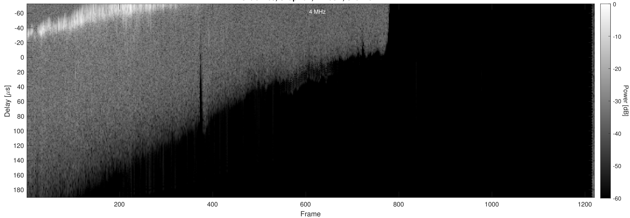
Orbit 7263, Chapman, Window, Channel 2
