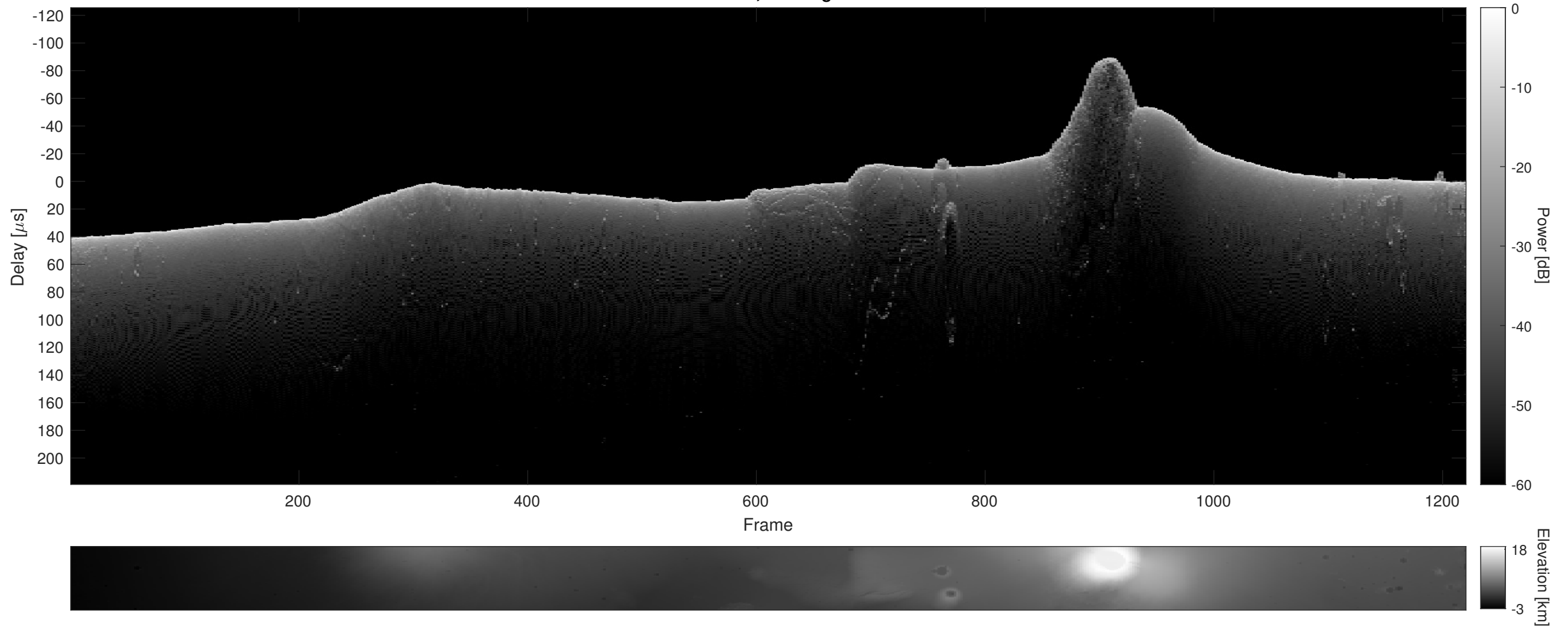
Orbit 7266, Cluttergram
