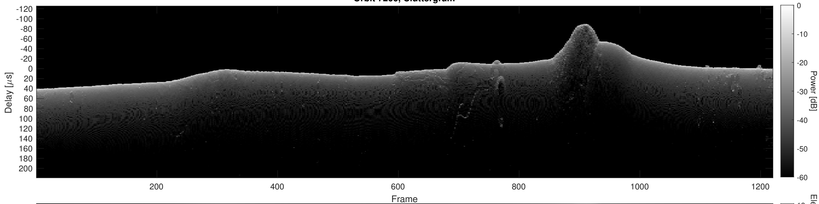
Orbit 7266, Cluttergram
