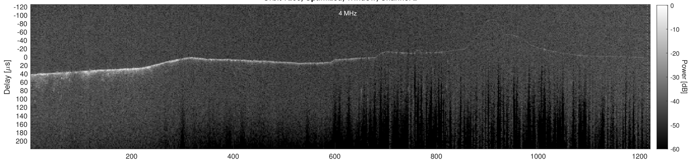
Orbit 7266, Cluttergram
