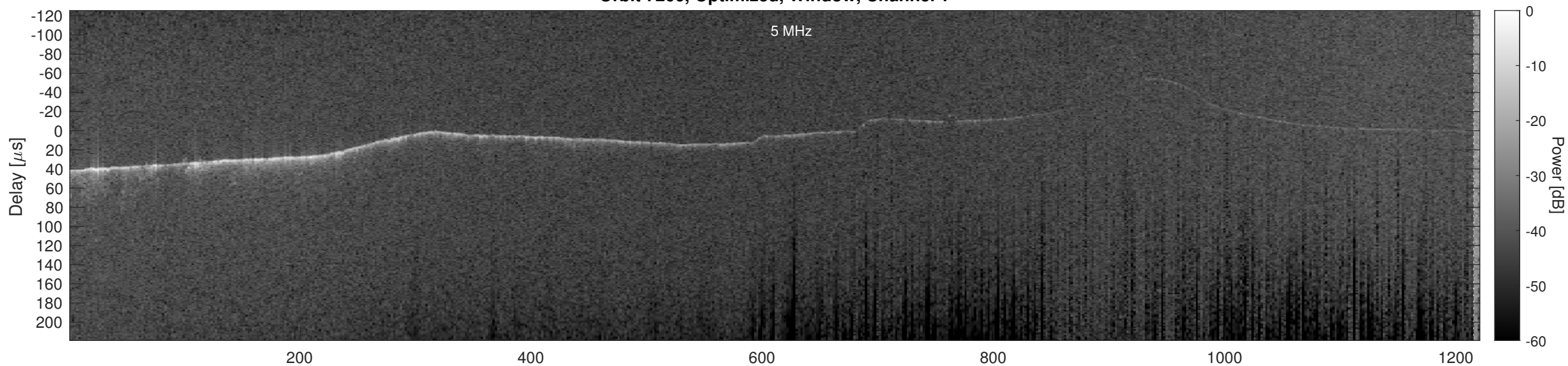
Orbit 7266, Optimized, Window, Channel 2
