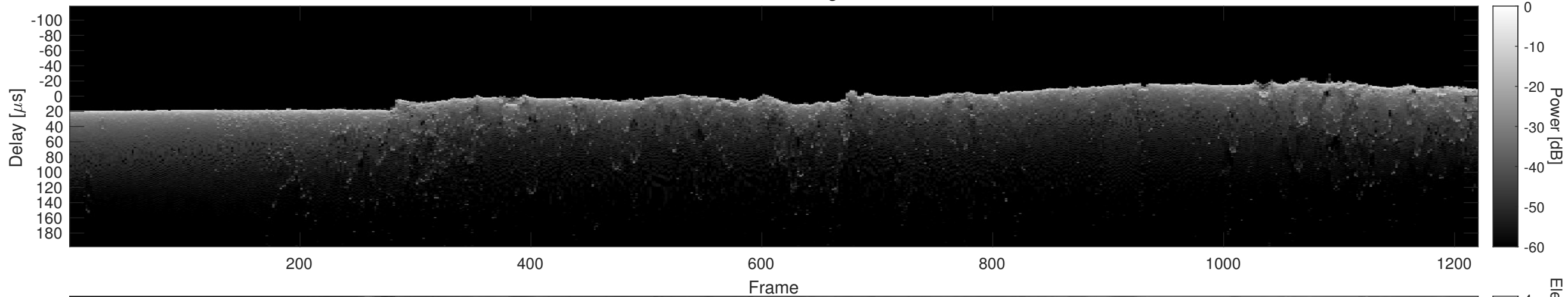
Orbit 7268, Cluttergram
