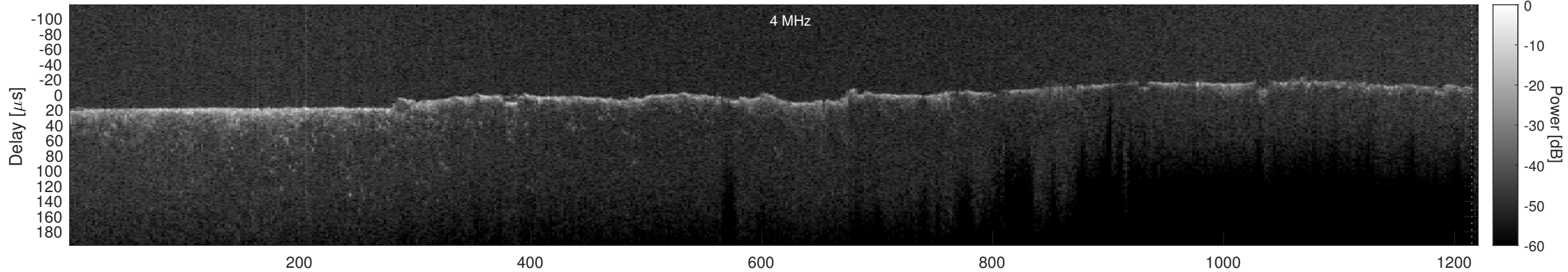
Orbit 7268, Cluttergram
