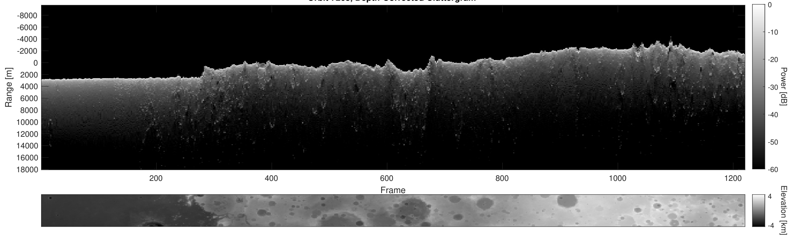
Orbit 7268, Depth-Corrected Cluttergram
