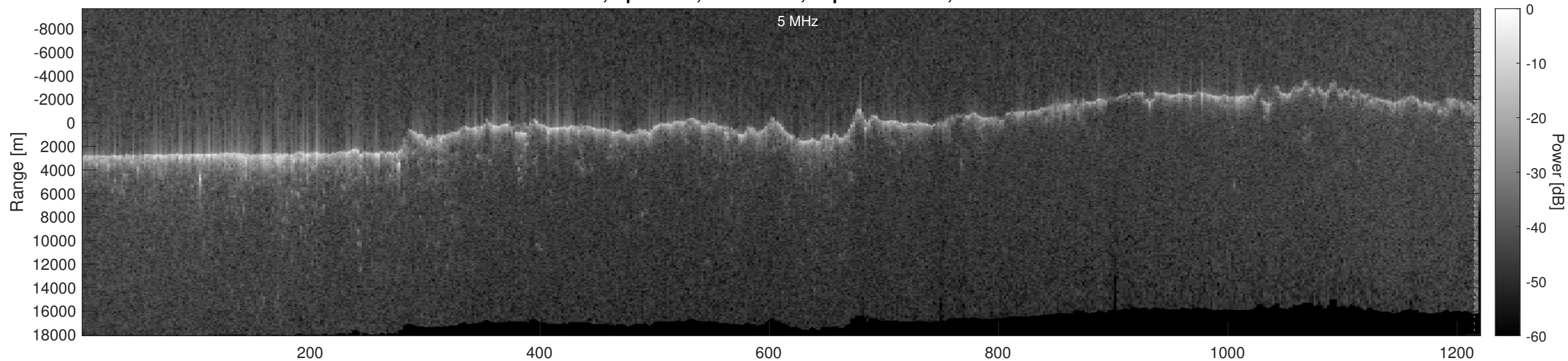
Orbit 7268, Optimized, No Window, Depth-Corrected, Channel 2
