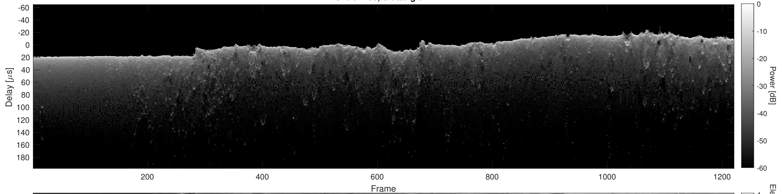
Orbit 7268, Cluttergram
