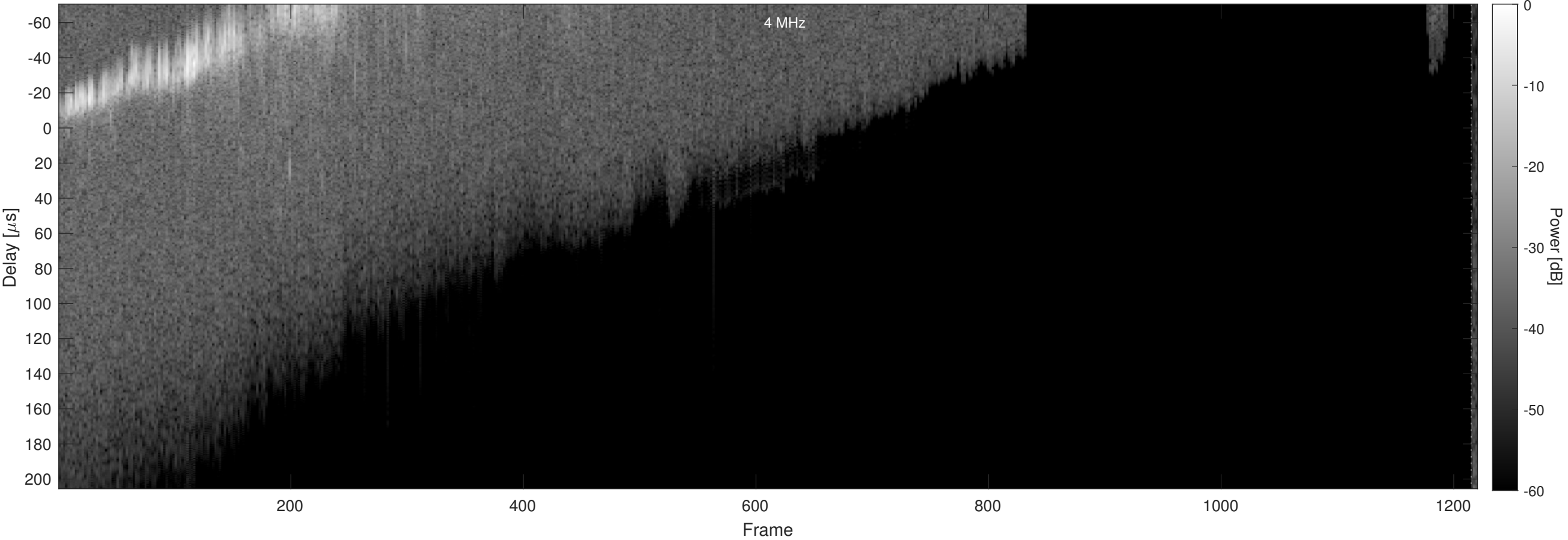
Orbit 7269, Chapman, Window, Channel 2
