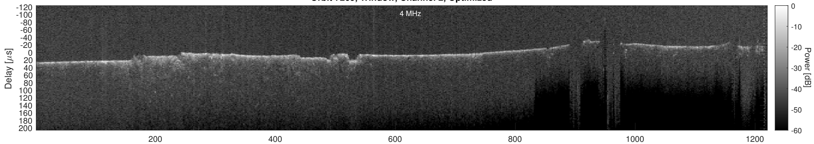
Orbit 7269, Cluttergram
