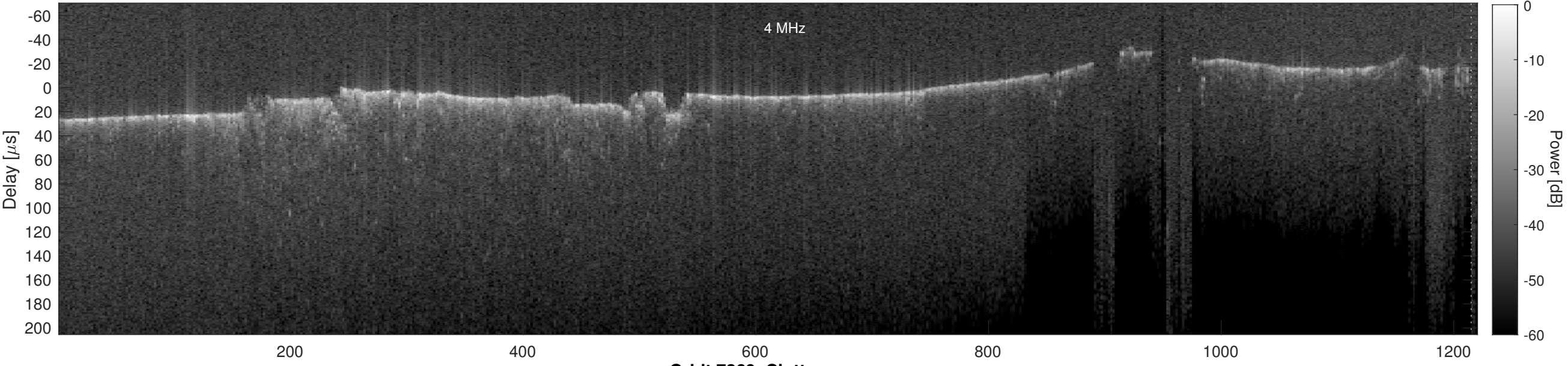
Orbit 7269, Cluttergram
