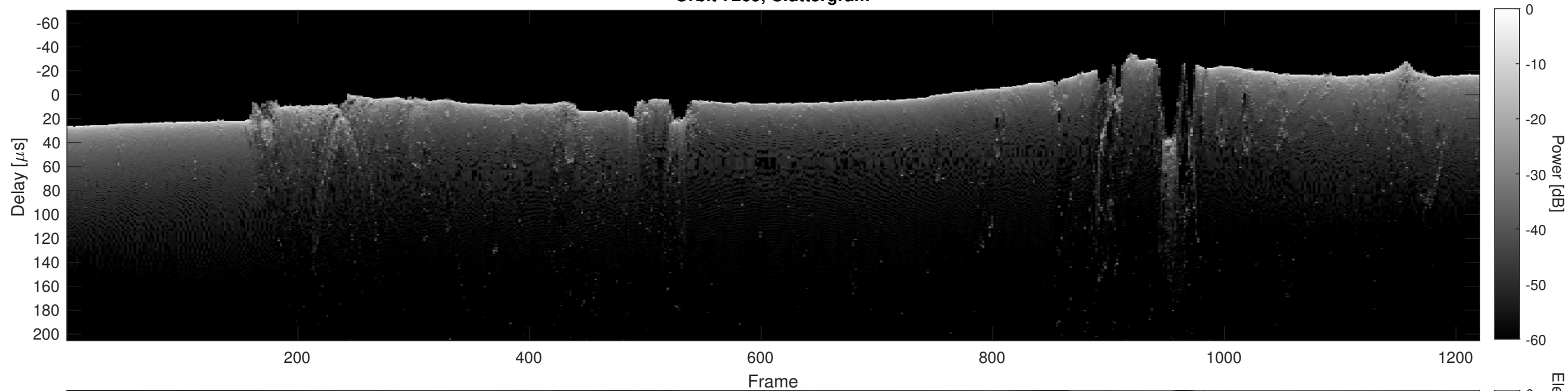
Orbit 7269, Cluttergram
