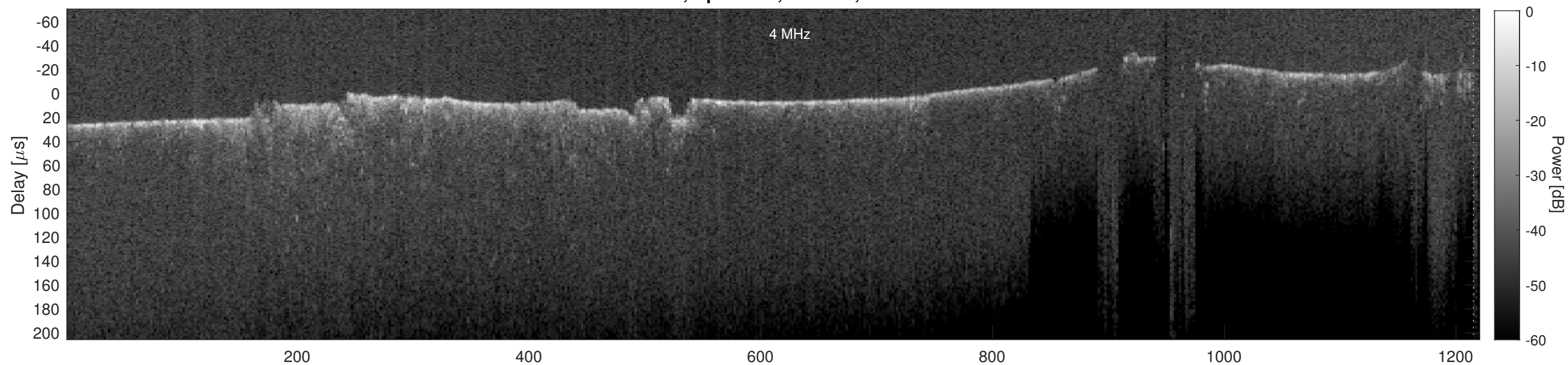
Orbit 7269, Cluttergram
