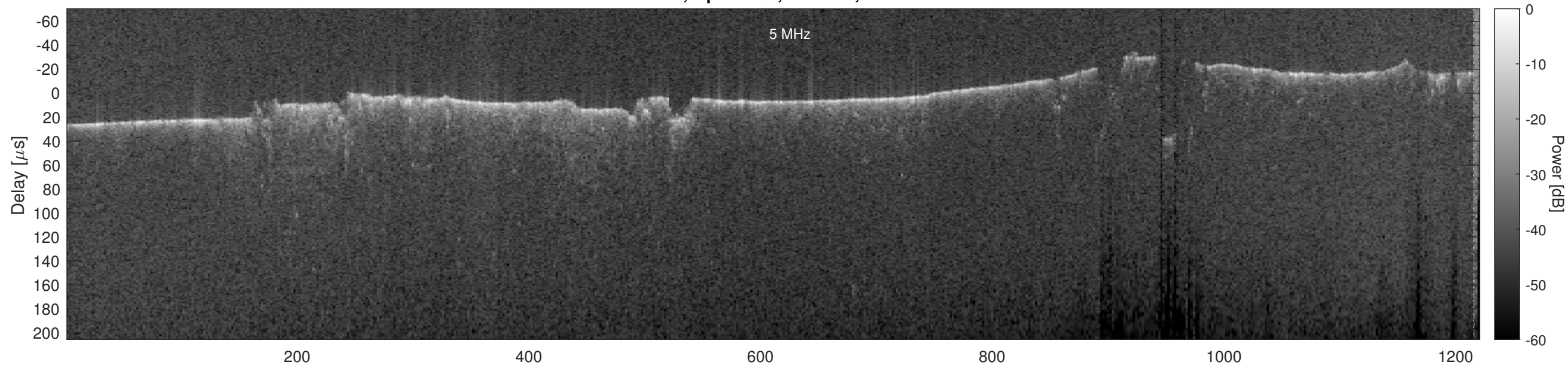
Orbit 7269, Optimized, Window, Channel 2
