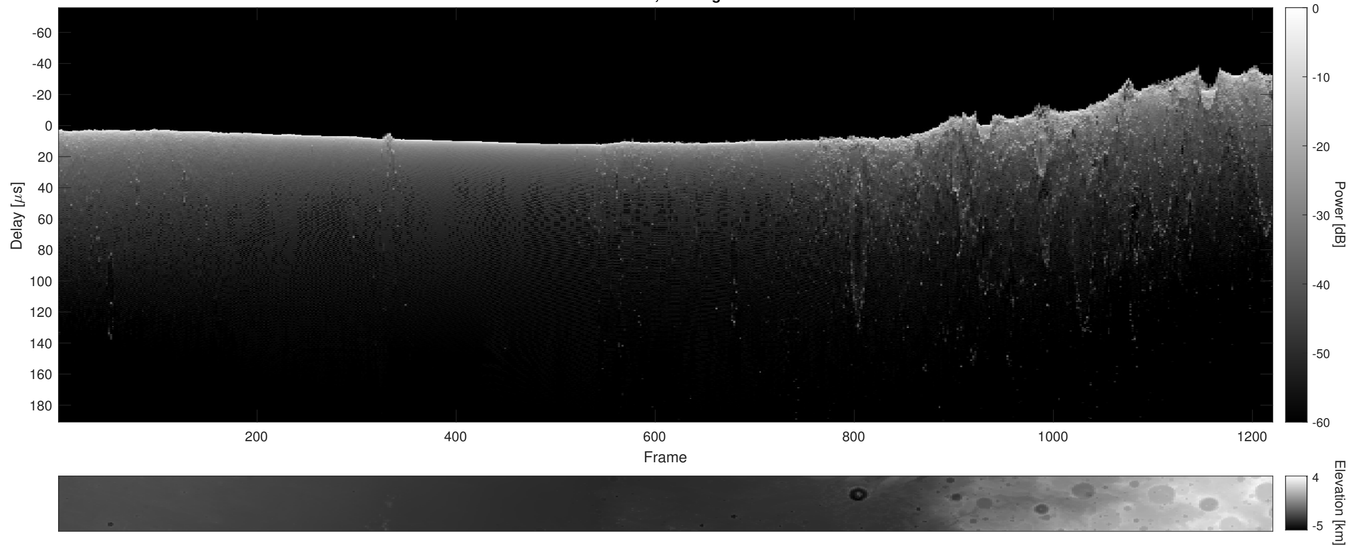
Orbit 7270, Cluttergram
